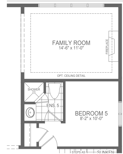
OPT. MAIN LEVEL
