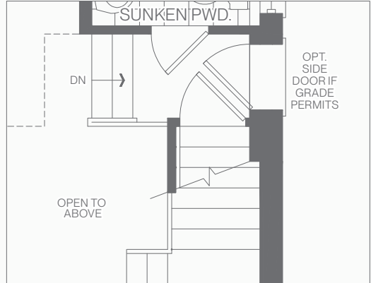
PARTIAL GROUND FLOOR PLAN W/OPT. SIDE DOOR ELEVATION A, B + C
