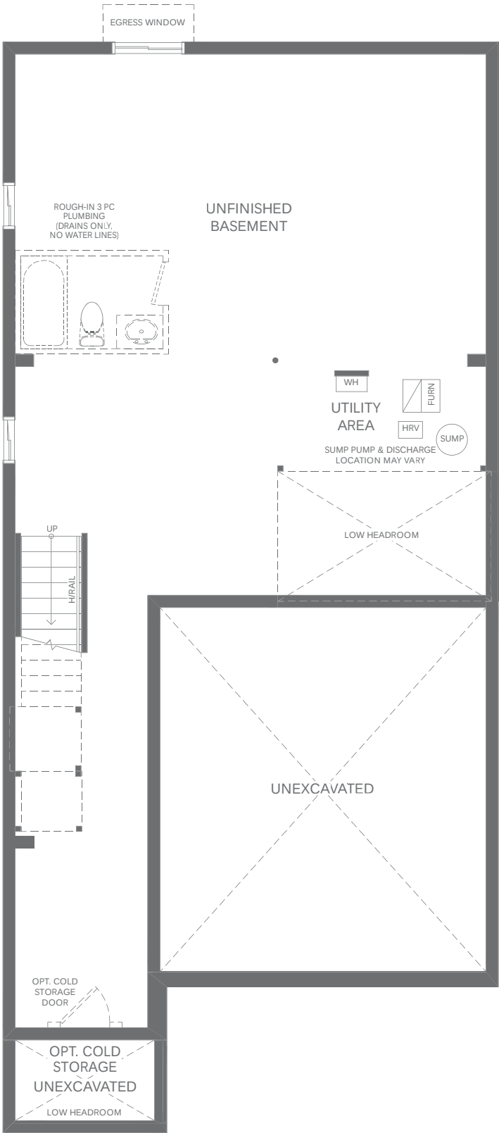
BASEMENT PLAN B
