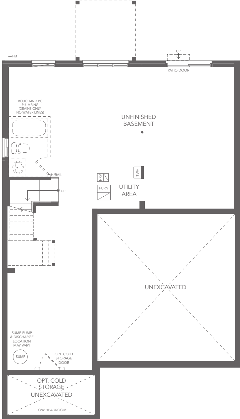
BASEMENT PLAN A
