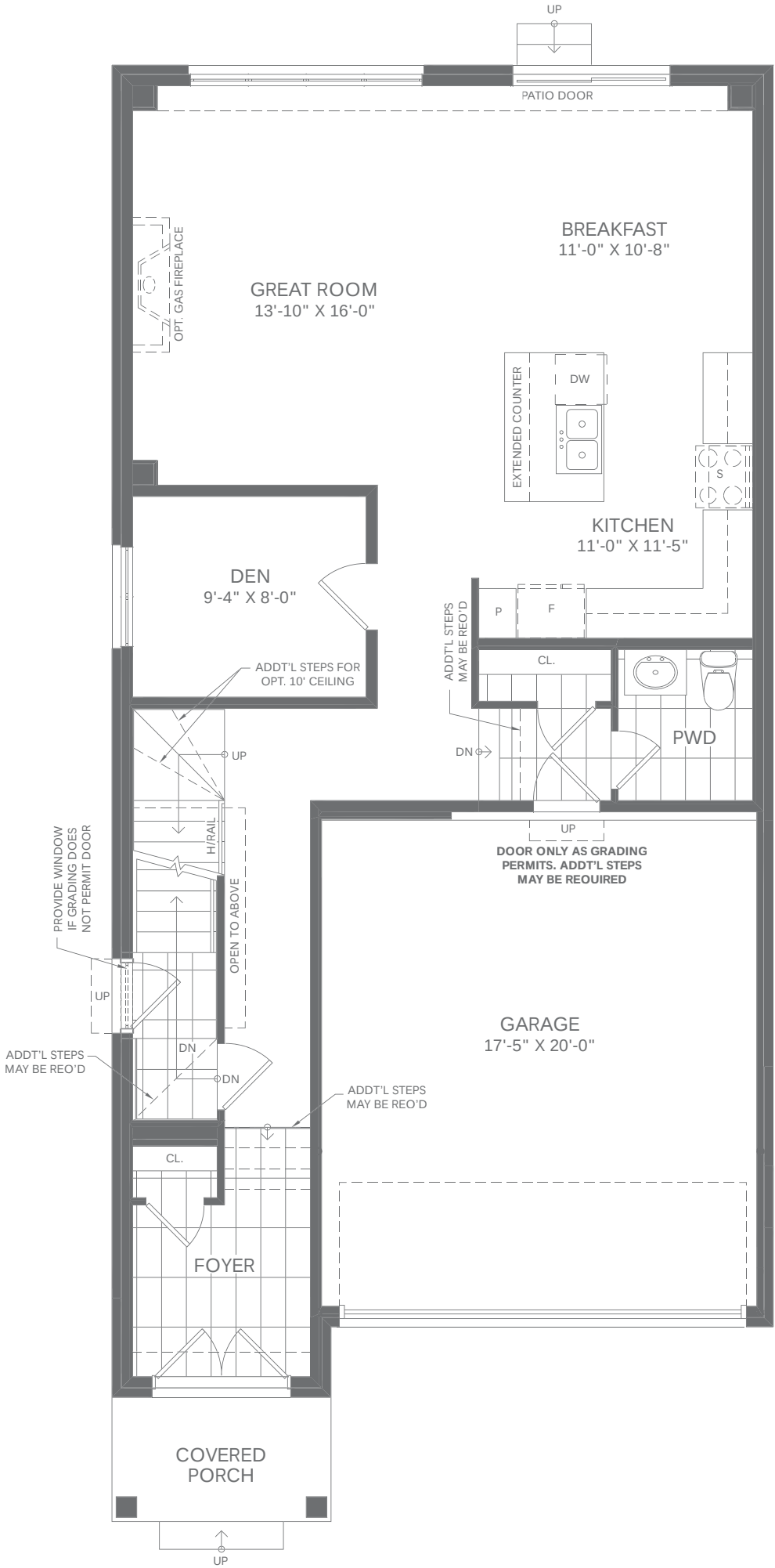
GROUND FLOOR PLAN B
