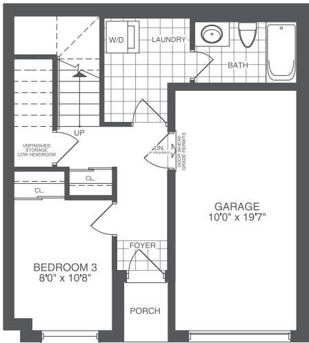
FIRST FLOOR ELEV. 1 & 2 FOR BUILDINGS M/N/P 1840 SF.
